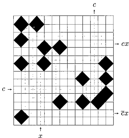
Fig. 18 A configuration of an S-gate in Model 2.
