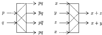
Fig. 5 An I-gate and an inverse I-gate.
