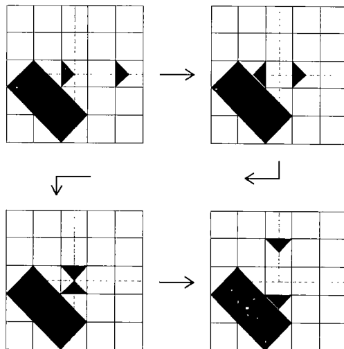
Fig. 12 Reflection of a signal by a mirror in Model 1.
