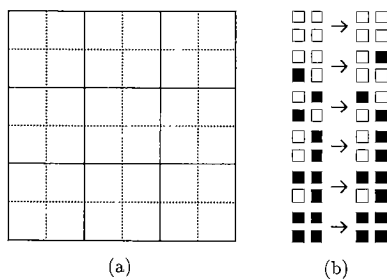
Fig. 2 (a) Margolus neighborhood. (b) The local function of the Margolus model.
