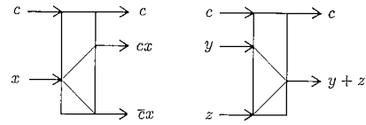
Fig. 6 An S-gate and an inverse S-gate.
